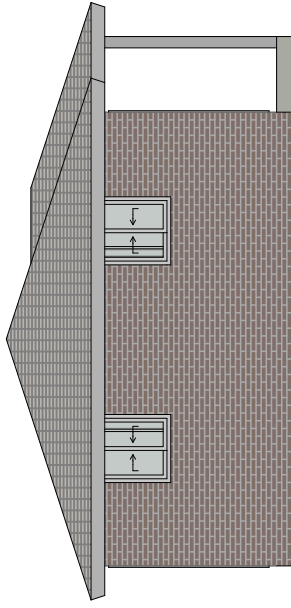
1:100 South Elevation
