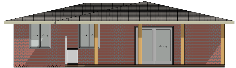
WEST ELEVATION 1:100
