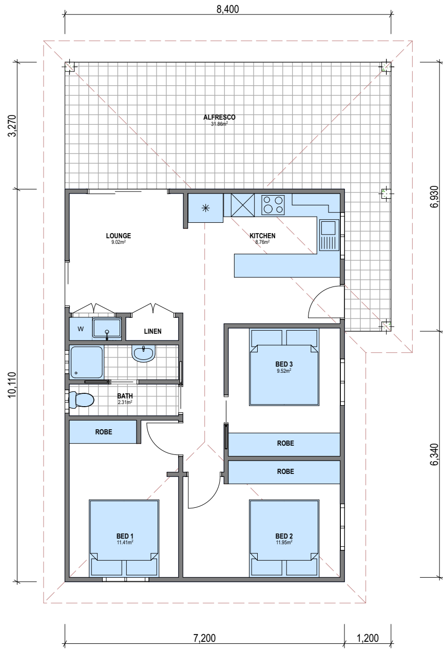
1. GROUND FLOOR PLAN 1:100
