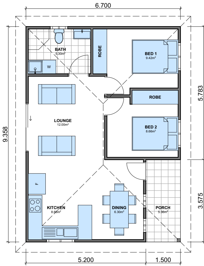
1:100 Ground Floor
