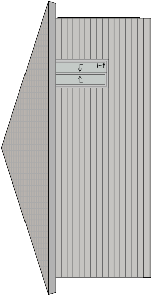
1:100 North Elevation
