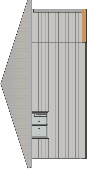
1:100 South Elevation
