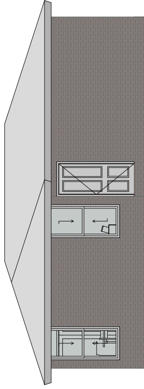
South Elevation 1:100
