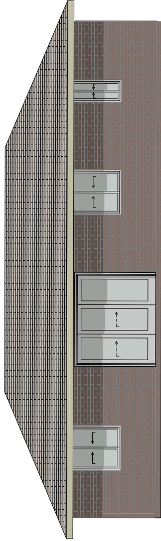
SOUTH ELEVATION 1:100
