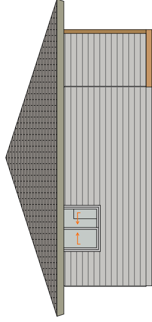
South Elevation
