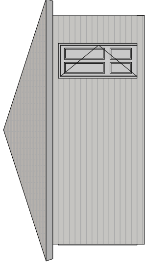
East Elevation 1:100
